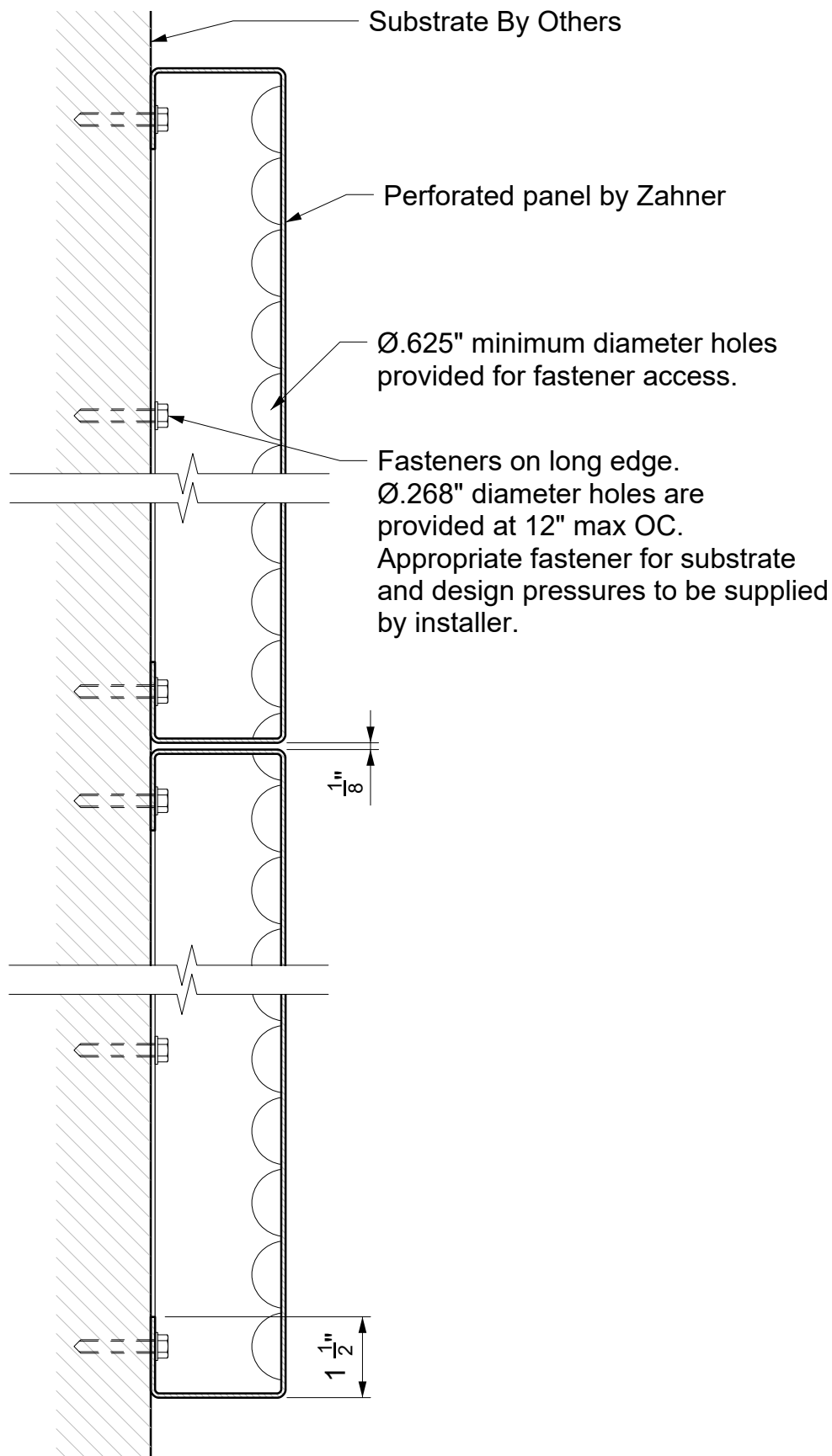
A-A Vertical Section 1" = 3"
