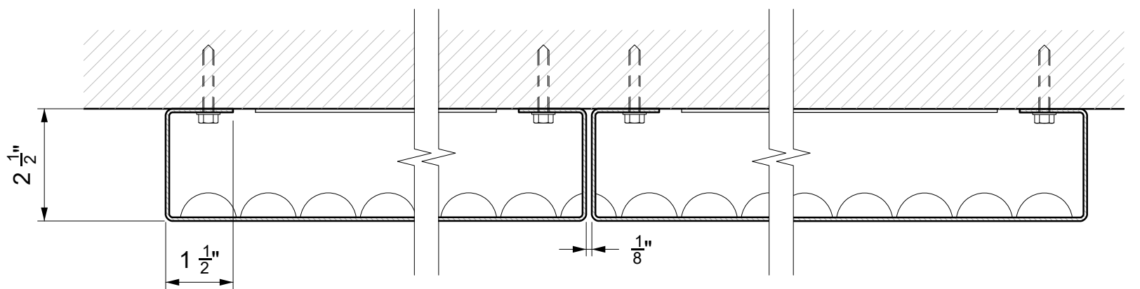
B-B Plan Section 1" = 3"
