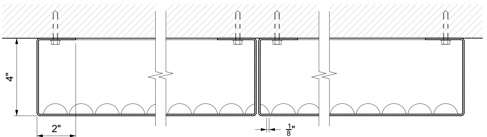
B-B Plan Section 1" = 3"
