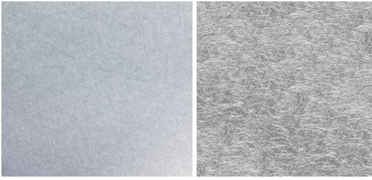
Left: Angel Hair Stainless Steel by Zahner. Above: "Vibration" finish by industry manufacturers. Right: The Zahner patented non-directional finishing system for manufacturing Angel Hair Stainless Steel.
